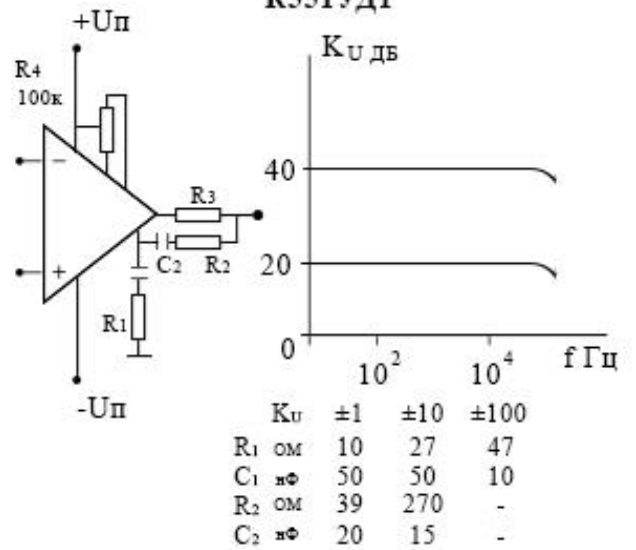
K551УД1
