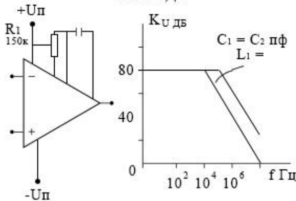
K544УД2
